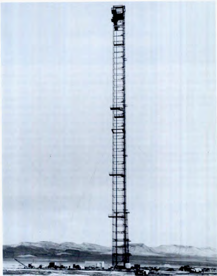
A test device mounted on a 500-foot tower at the Nevada Test Site. Taller and taller towers were built (to as high as 700 feet) to minimize entrainment of ground debris by the fireball and thereby reduce fallout resulting from the test.
